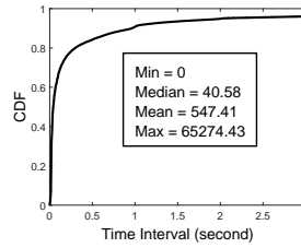
Figure 5: Time interval for SR/FF events.
