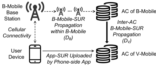
Fig. 2. Interactions among V-Mobile, its customers, and B-Mobile.
