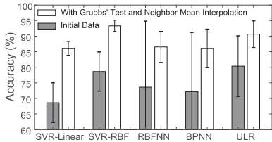
Fig. 10. Average prediction accuracy of different machine learning techniques.
