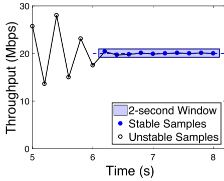
Fig. 2. Uplink test logic of FAST.
